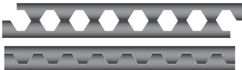
Figure 2. Manufacturing steel members with hexagonal web-castellation (Typical cut and reassembled castellated member)
