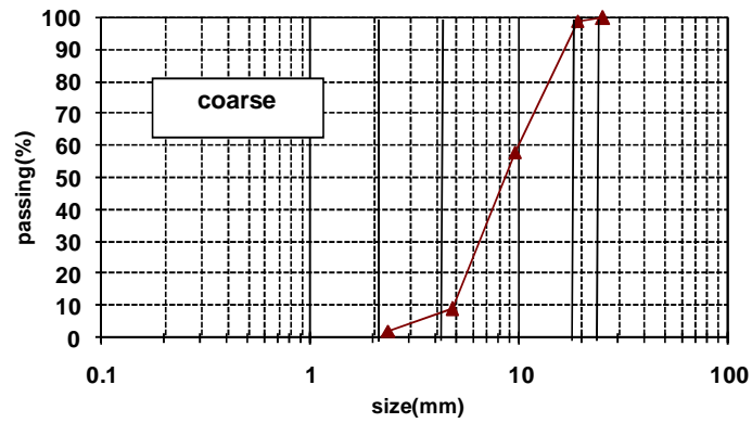
Figure 2. Curve of grading of coarse
