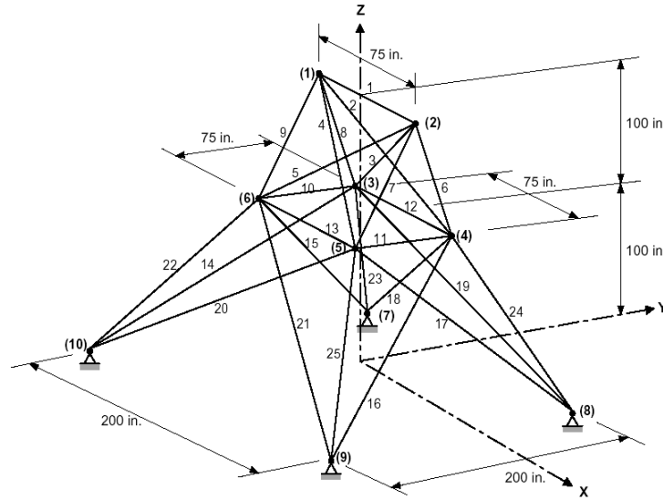
Figure 6. A twenty five-bar spatial truss
