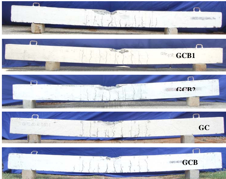
Figure 8. Crack pattern
