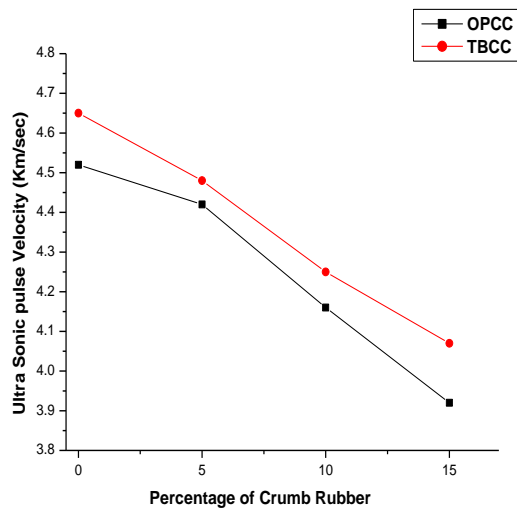
Figure 4. Variation of Ultrasonic Pulse Velocity of Concrete due to the addition of crumb rubber
