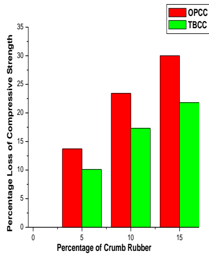
Figure 1. Variation of percentage loss of Compressive Strength of Concrete with crumb rubber
