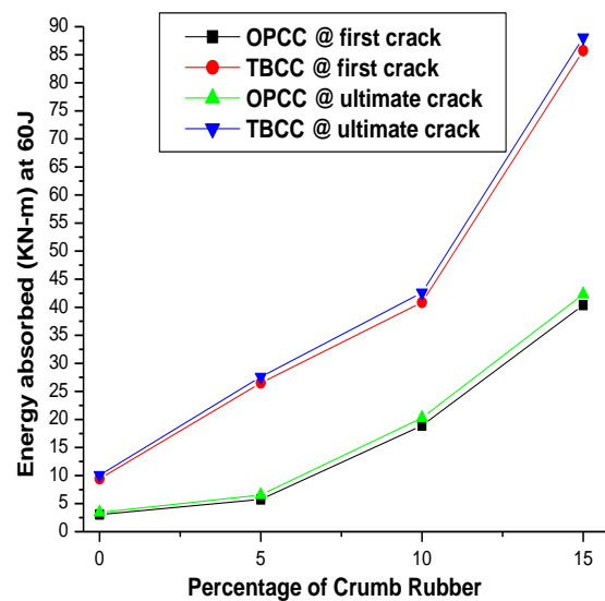
Figure 3. Variation of Impact Strength of Concrete due to the addition of crumb rubber
