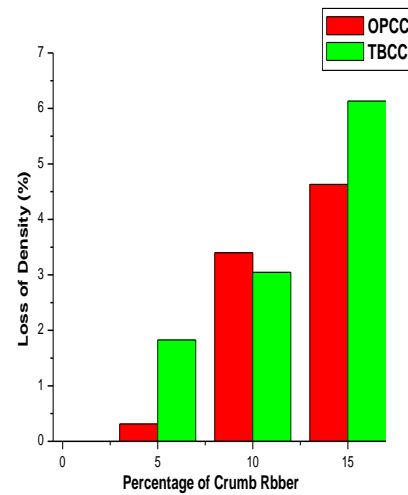
Figure 2. Variation of percentage reduction in density of concrete with crumb rubber
