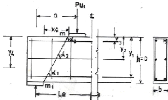
Figure 7. Notations in Kong, Robins and Sharp method
