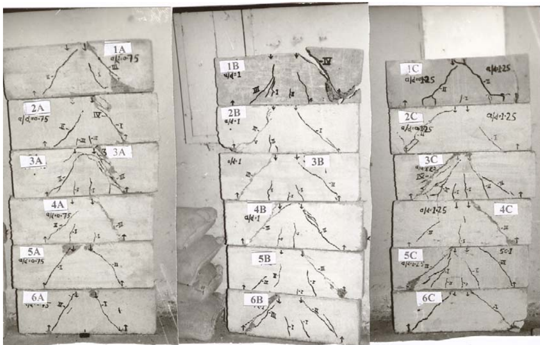
Figure 4. Cracking pattern and mode of failure for tested beams
