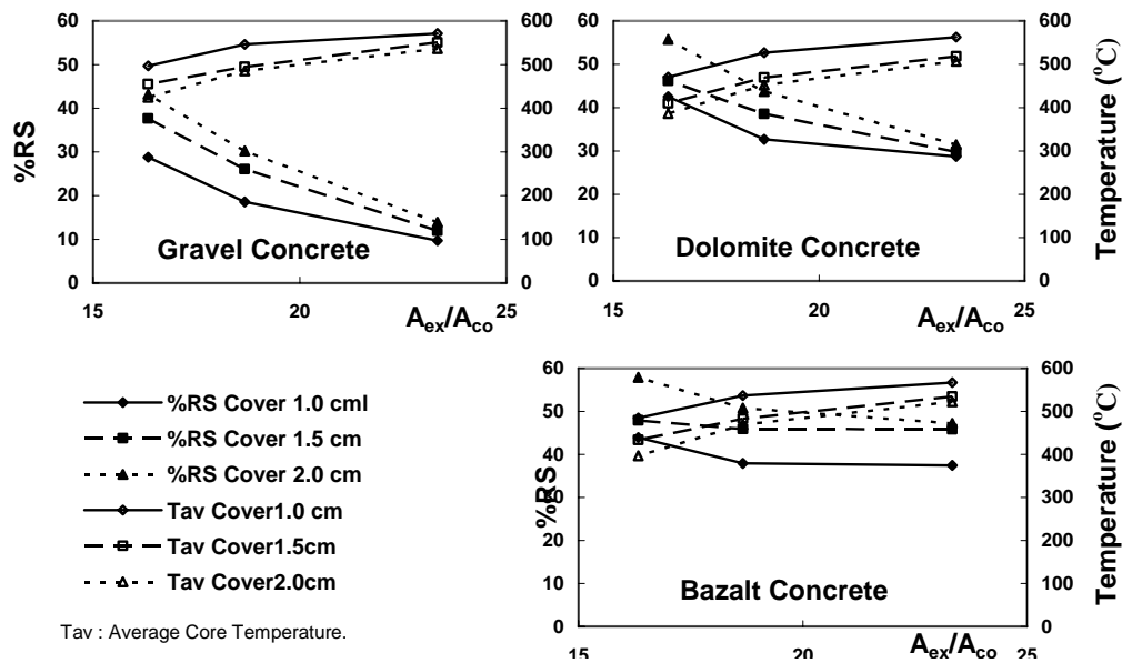
Figure 3. Average core temperature /residual strength versus the ratio of exposed area to cross sectional area for different concrete cover and aggregate type
