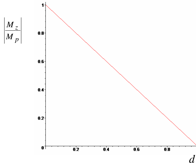
Figure 6. Yield function Z_{Md}
