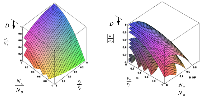
Figure 4. Yield surface for rectangular cross section depending on the stresses and damage Z_{MNVd}
