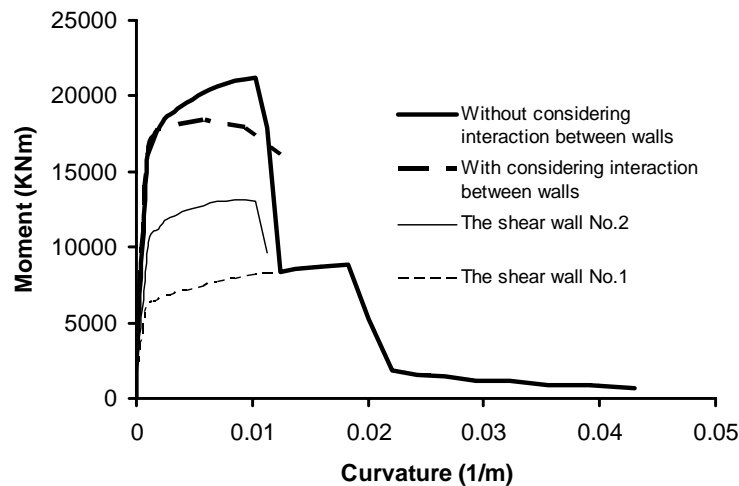
Figure 14. The moment-curvature under axial force and flexural moment
