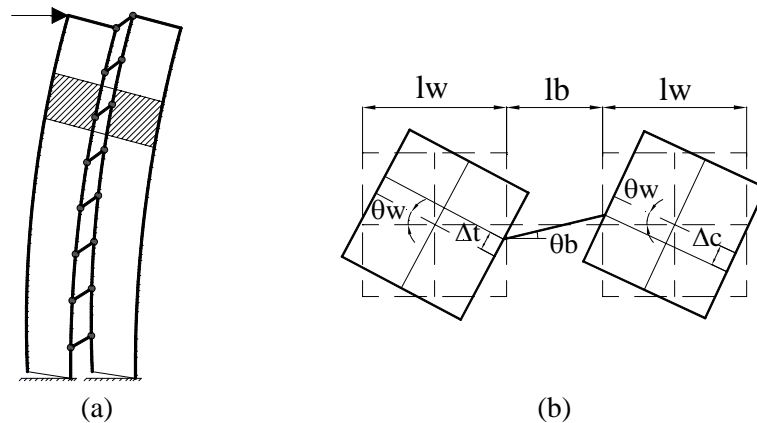
Figure 5. (a) Deformation of coupled shear walls due to the lateral load (b) Plastic deformation of link beam
