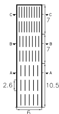
Figure 9. Geometric dimensions of slit shear walls (dimensions in meters)
