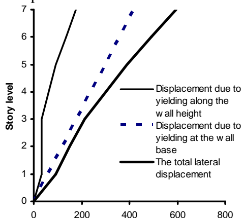
Figure 10. Lateral displacement in the slit shear walls
