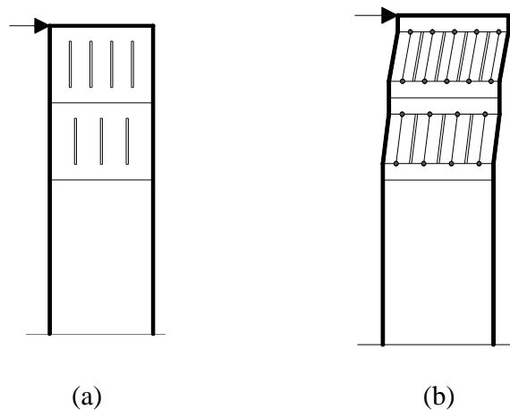
Figure 8. (a) Slit shear walls with shear mode deformation (b) Plastic mode deformation
