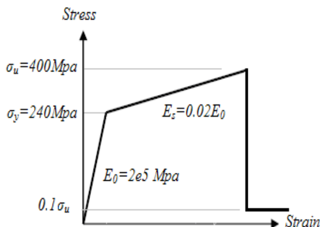
Figure 8. Stress-strain curve for steel parts of the models (frames and steel walls)
