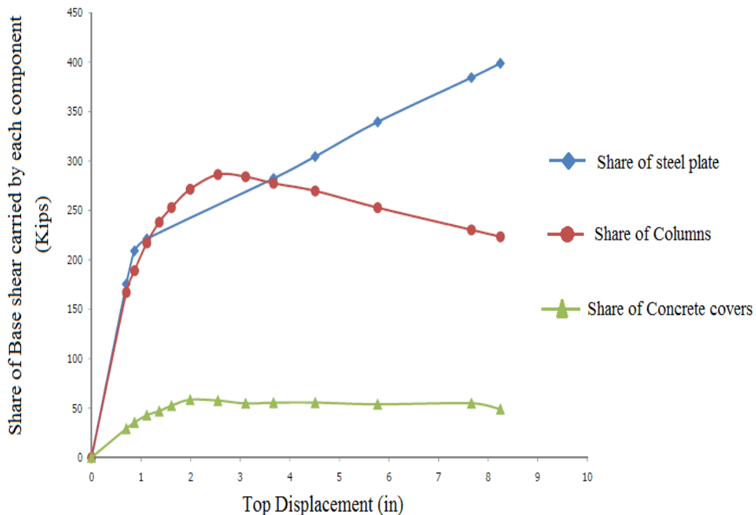
Figure 6. Proportion of base shear carried by each component of the system
