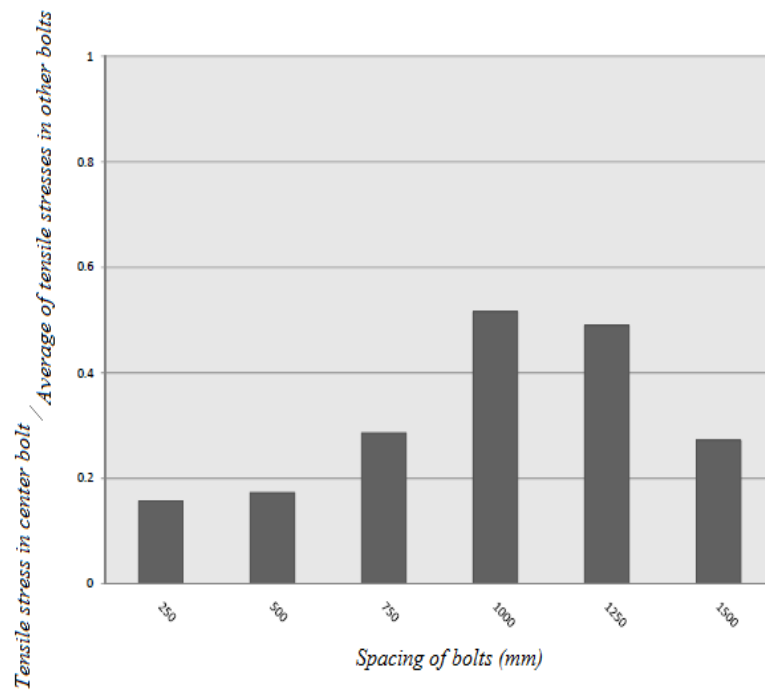
Figure 14. Comparing the ratio of tensile stress in center bolt divided to average of tensile stresses obtained in other bolts
