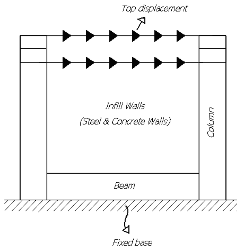
Figure 2. A schematic illustration of loading condition
