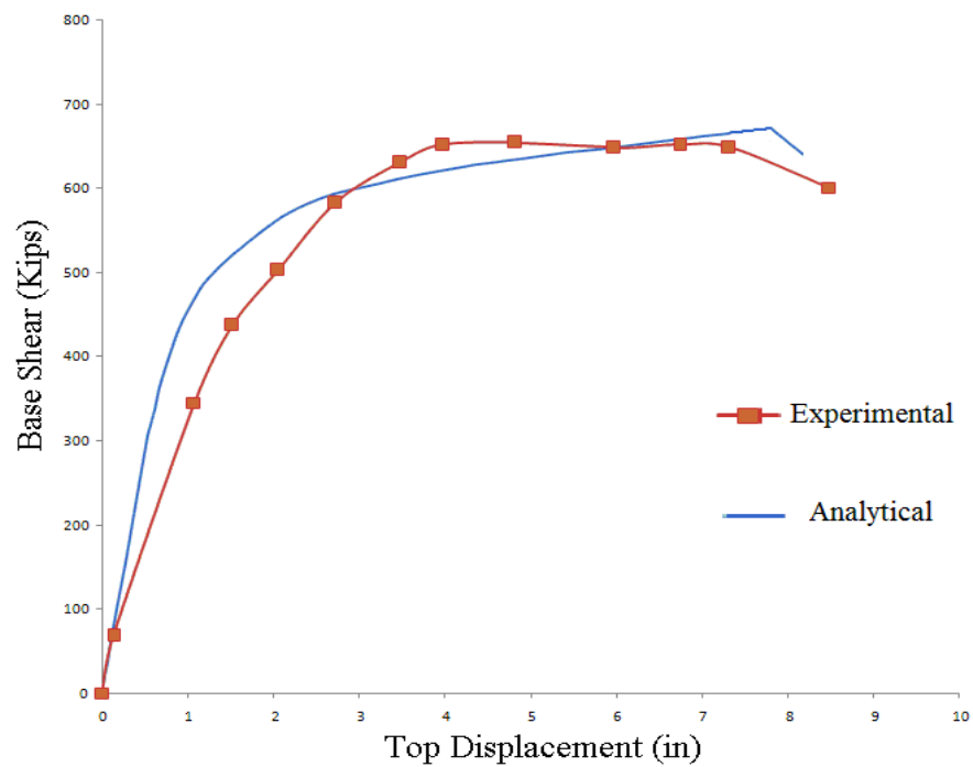
Figure 4. Comparison of experimental and analytical curves of Astenh specimen
