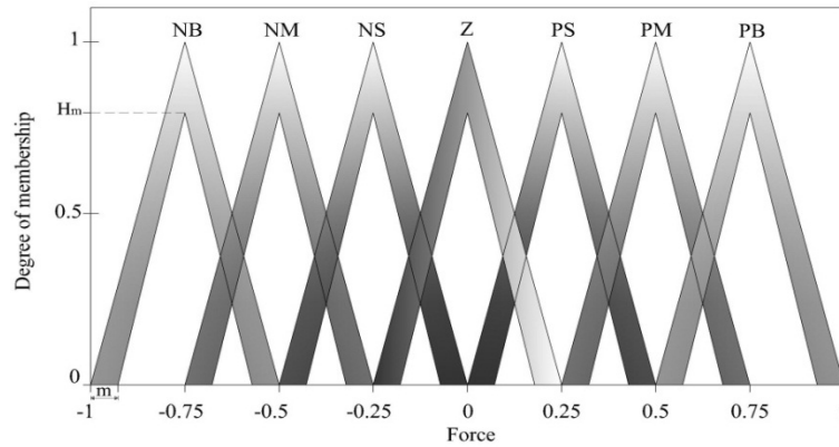
Figure 5. MFs of output variable (active control force)
