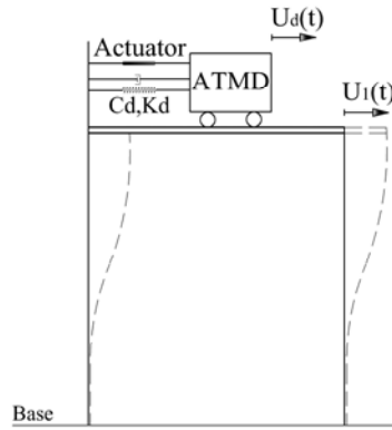
Figure 1. SDOF system with ATMD
