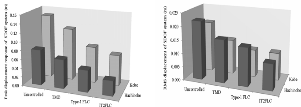
Figure 6. Controlled and uncontrolled peak displacement response and RMS displacement of SDOF system under the Kobe and Hachinohe earthquake records
