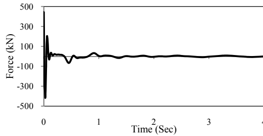
Figure 11. Fuzzy control stability test in terms of control force
