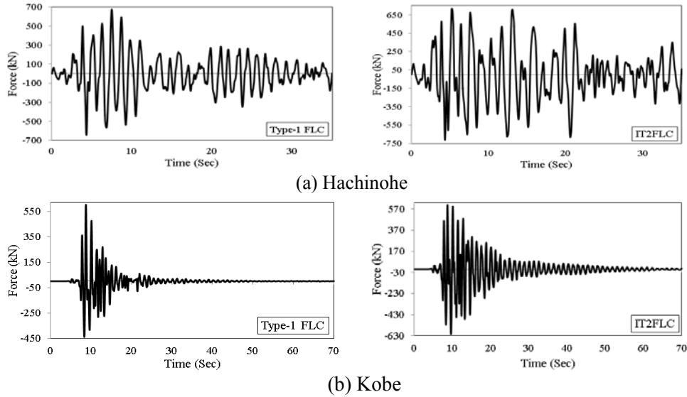
Figure 10. Comparison between the active control forces needed in type-1 FLC and IT2FLC for the Hachinohe and Kobe earthquakes
