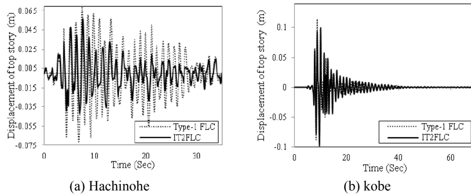
Figure 8. Comparison of displacement time history responses of the top story for different control systems under the Kobe and Hachinohe earthquake records
