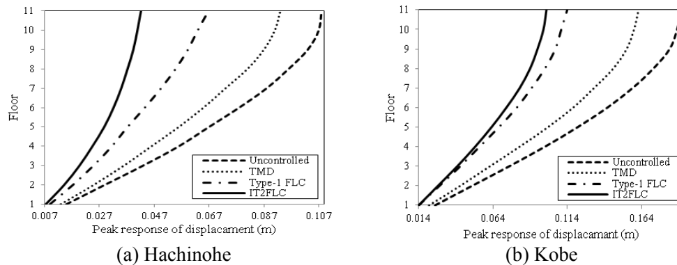
Figure 7. Controlled and uncontrolled peak displacement responses of floors
