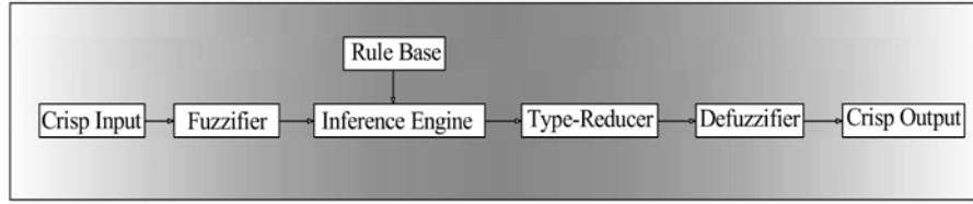
Figure 3. IT2FLS structure
