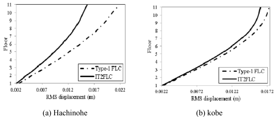
Figure 9. Comparison of RMS displacement of stories in case of using type-1 FLC and IT2FLC
