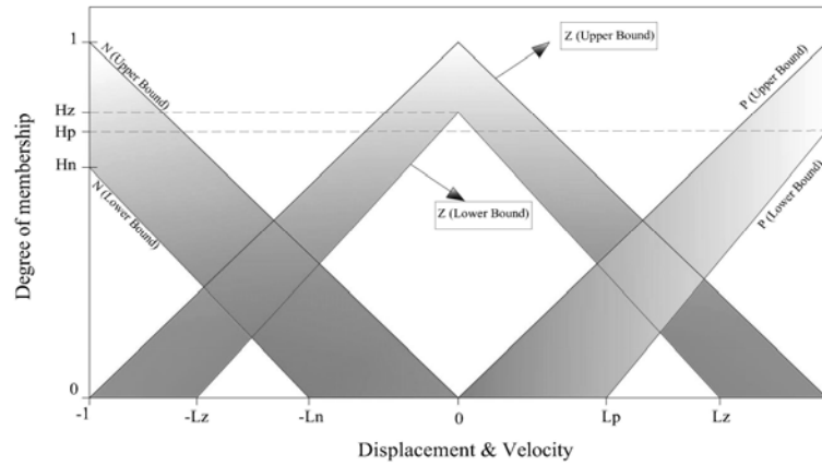
Figure 4. MFs of input variables (displacement and velocity)
